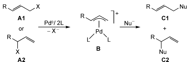
Scheme 1. Simplified mechanism of the Tsuji–Trost reaction.
