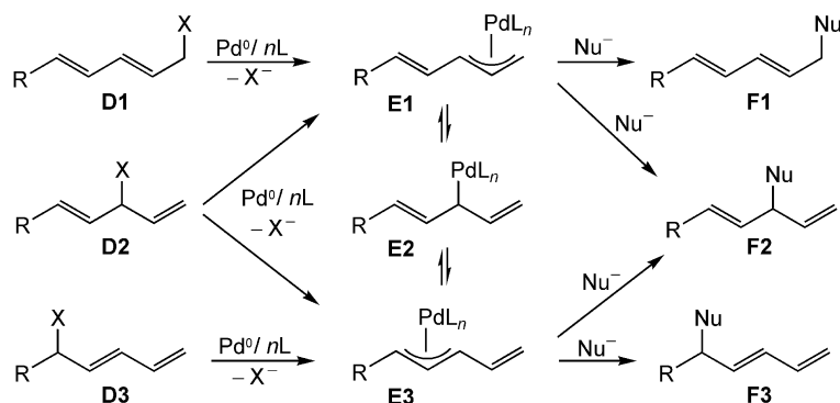
Scheme 4. Allylic alkylations with dienyl substrates D .
