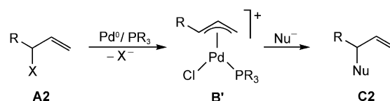
Scheme 2. Formation of unsymmetrical ( \pi -allyl)palladium complexes.
