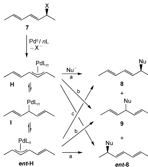
Scheme 7. Formation of isomeric products from optically active 7 .
