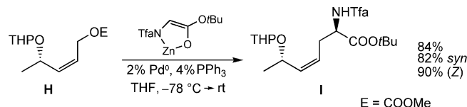
Scheme 5. Allylic alkylations of chelated enolate G (Tfa = trifluoroacetyl).
