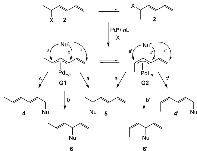
Scheme 6. Formation of isomeric products 4–6 from allylic substrate 2 .
