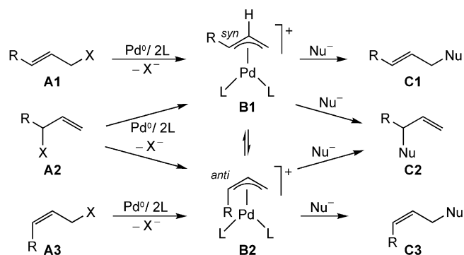
Scheme 3. Detailed mechanism of allylic alkylation.
